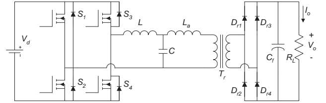
Fig. 2: Circuit diagram of full-bridge LCL-T resonant converter.
